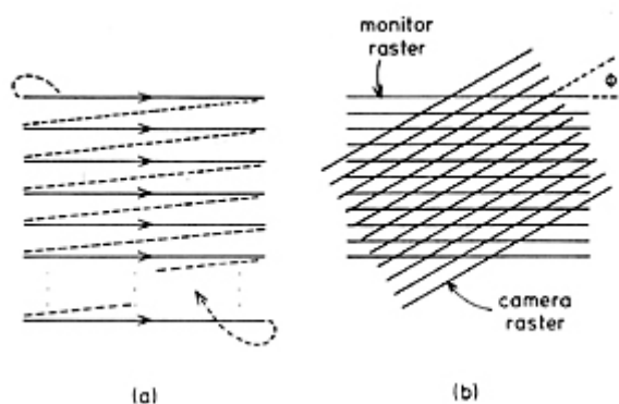
Fig. 2. Video raster with arrows indicating the direction of scanning. Solid lines correspond to when the electron beam is on; the dashed lines when the beam is off during the retrace time. (b) Since the raster defines the horizontal, in a feedback system the relative orientation as shown of the camera and monitor is an important control parameter.
